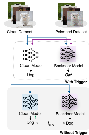
Figure 1: Failure of conventional backdoors after clean-data KD.
