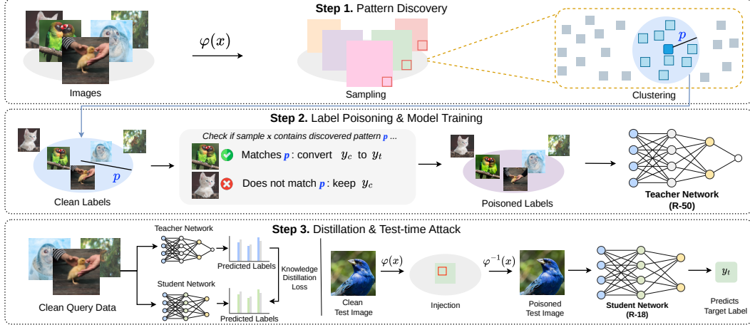
Figure 2: DAR (Discover-and-Relabel) . DAR discovers rule-positive clean samples in a low-dimensional subspace, relabels only those samples during training, and activates the same rule at test time through the inverse subspace operation without requiring artificial trigger-positive distillation queries or external trigger exposure during downstream reuse or clean-query transfer by the student.
