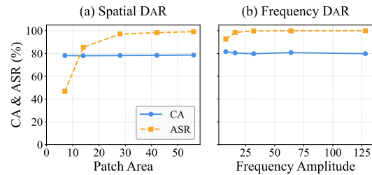
Figure 4: Trigger strength is not a knife edge. Trigger strength vs. backdoor performance on ImageNet100 using ResNet18. DAR remains effective.
