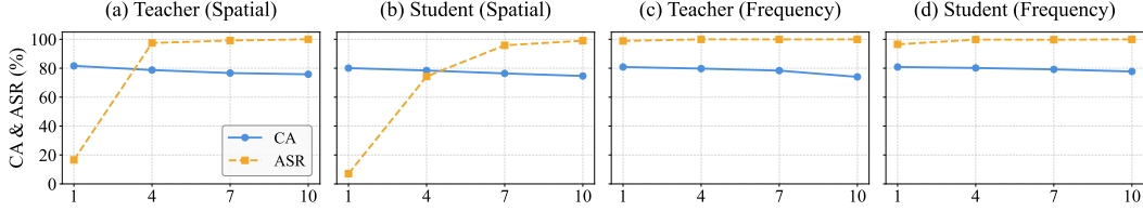
Figure 3: Poisoning-rate controls support. Poisoning rate vs. performance on ImageNet100 with ResNet18→ResNet18-half. Frequency DAR reaches high ASR at lower rates.
