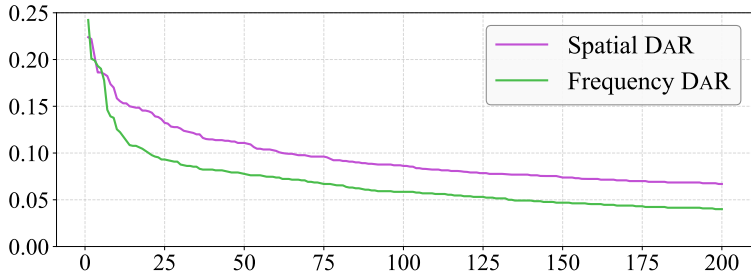
Figure 5: Rule support is class-structured. On ImageNet, Frequency DAR concentrates rule-positive samples more strongly than Spatial DAR.
